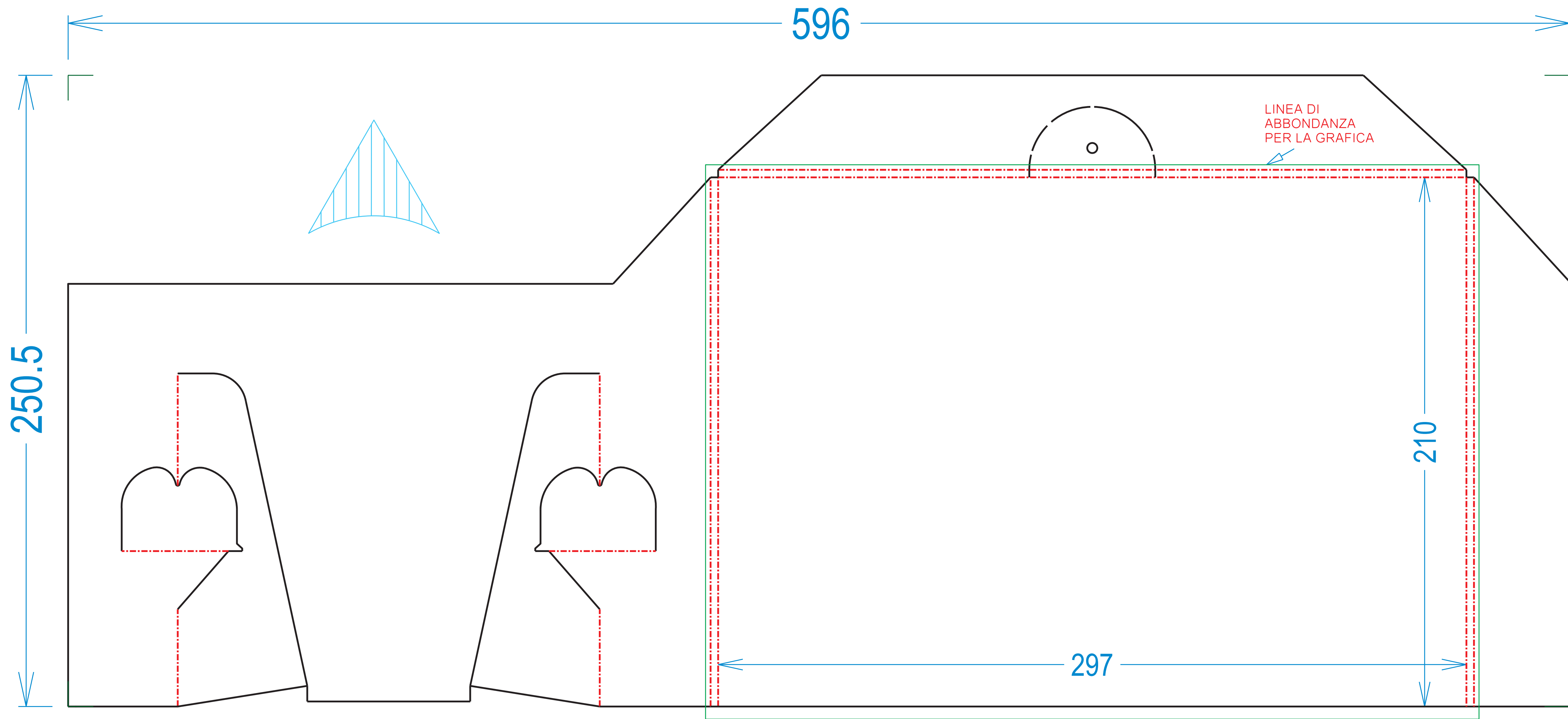
PINZA LATO STAMPA COD. 800_3003-06_DIS1
